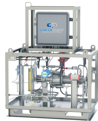
IntellijECT PLC controlled fully automated portable 8400 high pressure injection package with local, remote and automated flow control with flow, pressure and temperature transmitters, actuated discharge ball valve and fire fuse for emergency shutdown. Class 1, Div 1. Final destination: GOM
