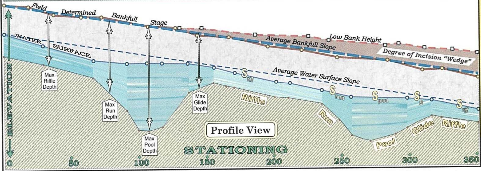
Figure 2-10. Plan and profile views of a longitudinal profile indicating max depth and facet slope measurement locations. Note: Stationing distance in this example is measured
